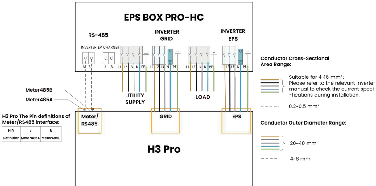
Wiring diagram with H3 Pro
