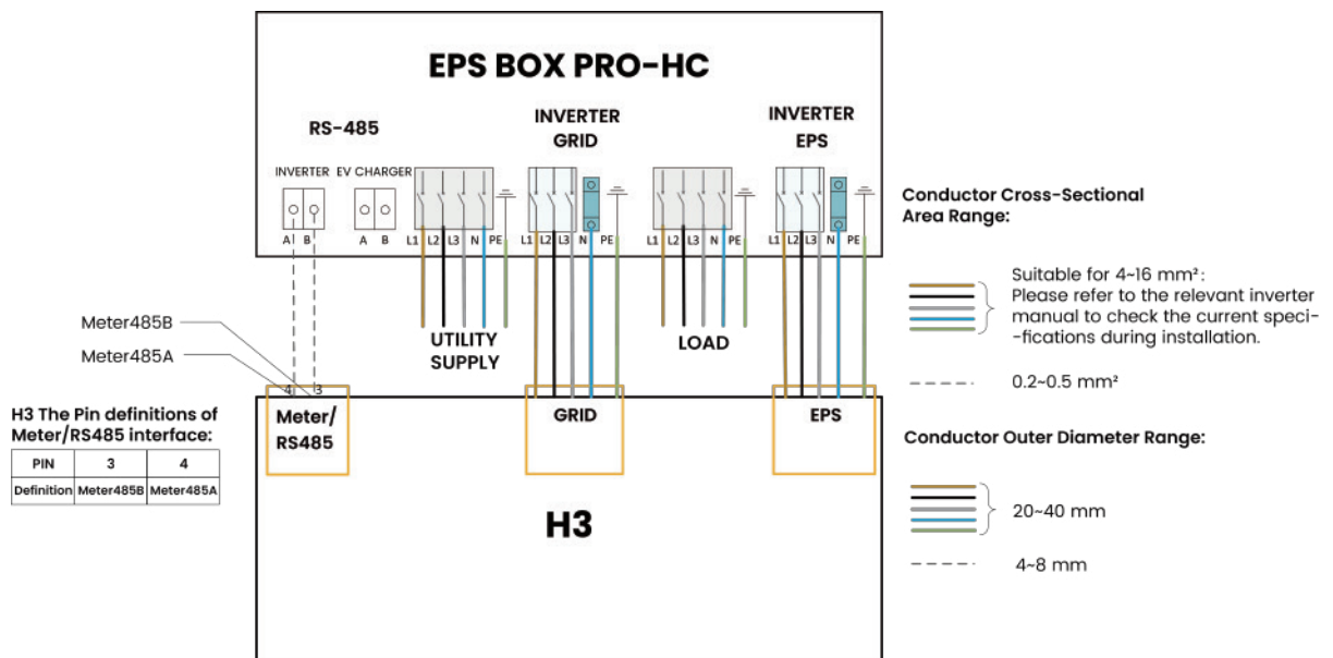
Wiring diagram with H3
