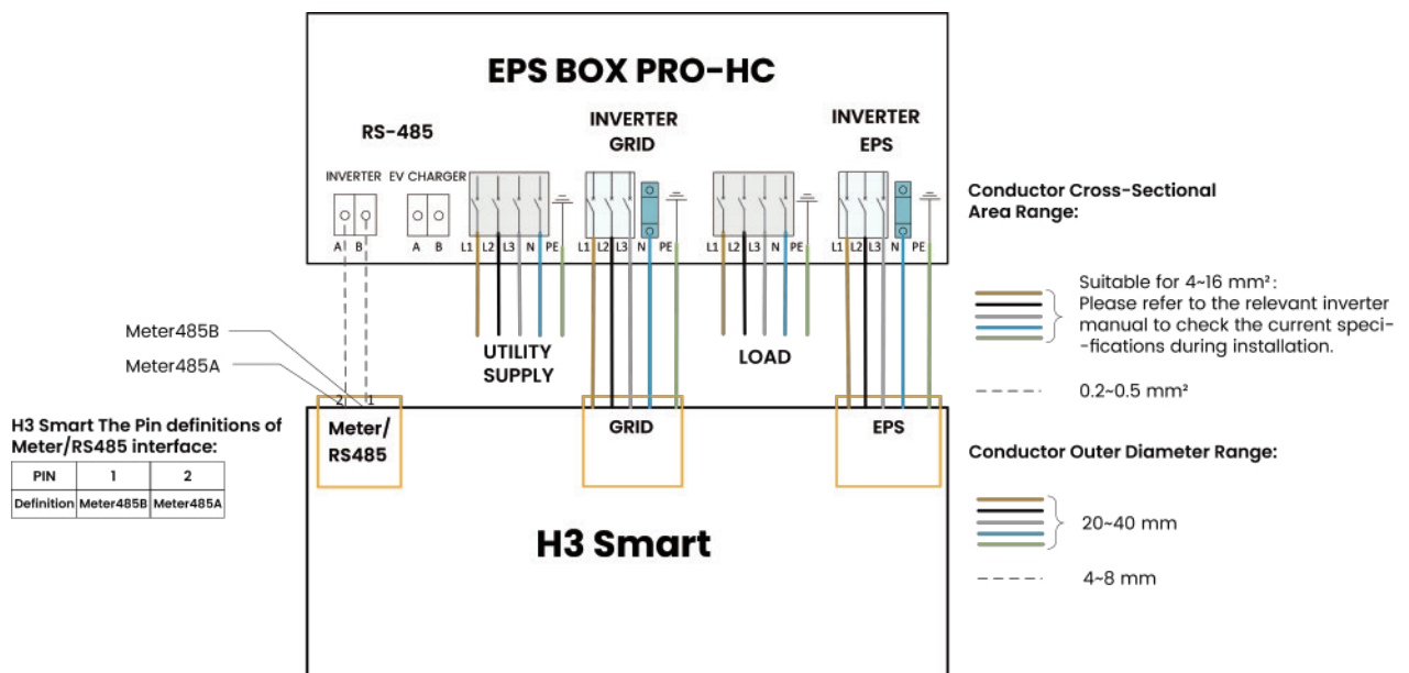
Wiring diagram with H3 Smart
